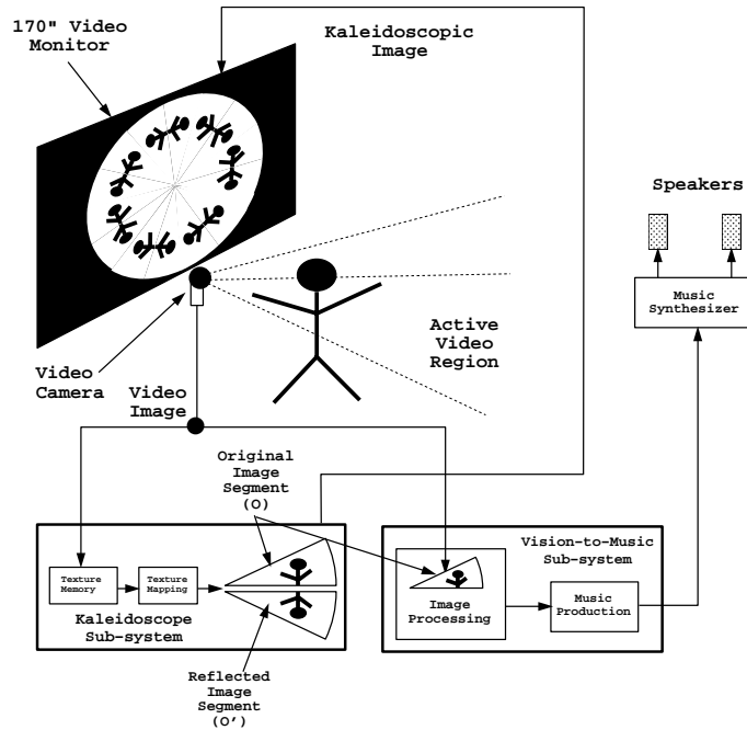
Figure 2: Block diagram of the Iamascope. Output from the video camera feeds into both the kaleidoscope sub-system and the vision-to-music sub-system. The kaleidoscope sub-system places the video image into texture memory and extracts the root image to form the kaleidoscope. Texture hardware performs the mirror reflections and the output is displayed on the large screen. The vision-to-music sub-system uses the same root image as input and performs motion analysis on sub-sections of the root image. The output from the motion analysis is processed and converted to MIDI signals to control a MIDI synthesizer. The kaleidoscope sub-system runs at 30 fps on an SGI Onyx with a Sirius video option and the vision-to-music sub-system runs at 15fps on an Indy.
