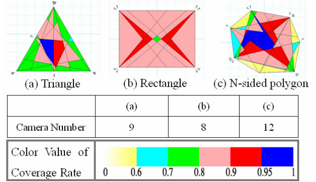
Figure 10 Camera Configurations for Various Polygons
